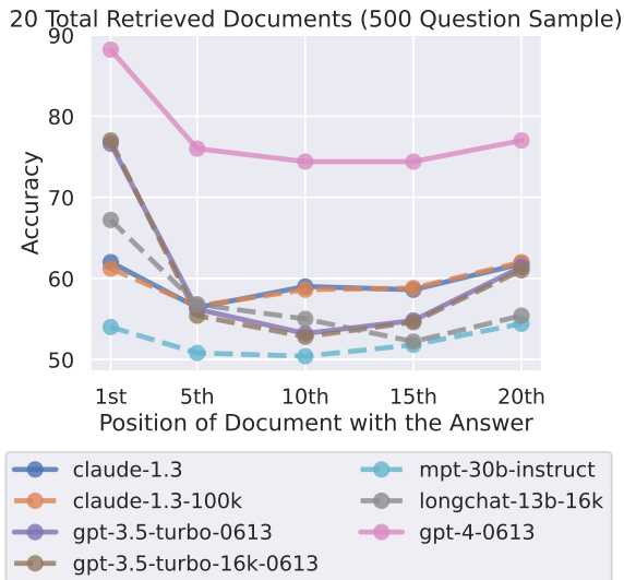
Figure 17: Although GPT-4 has higher absolute performance than other models, its performance still degrades when relevant information occurs in the middle of the input context.
