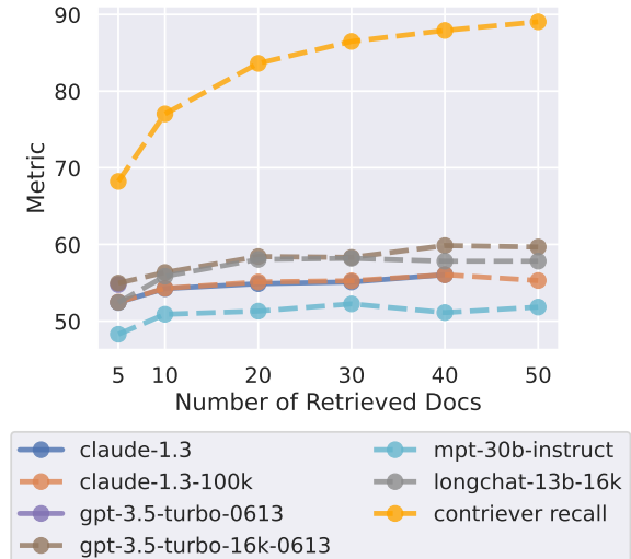
Figure 14: Retriever recall and model performance as a function of the number of retrieved documents. Model performance saturates long before retriever performance levels off, indicating that the models have difficulty making use of the extra retrieved documents.
